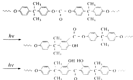
Fig. 1. Photo-Fries rearrangement of polycarbonate.
