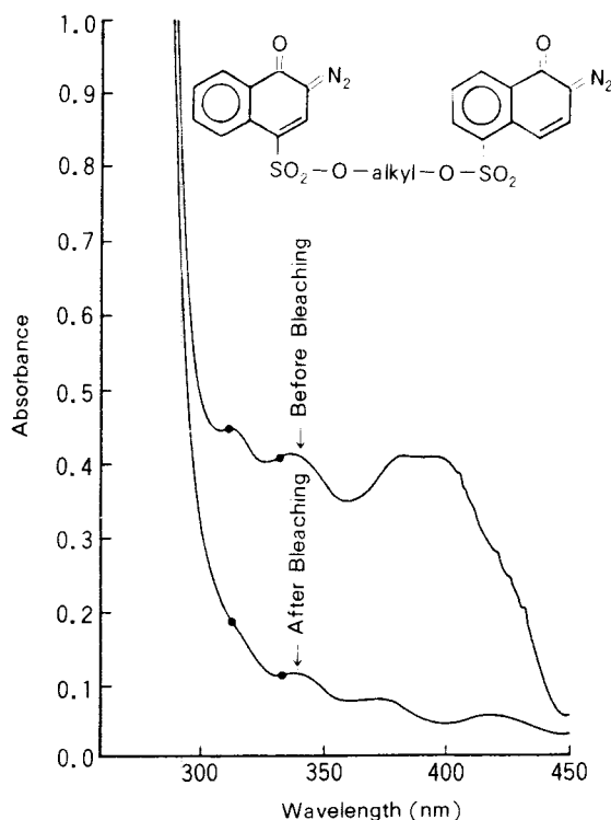
Fig. 10. Unexposed and bleached spectra of an IBM mid-UV resist formulated from a 4,5-disulfonate of an aliphatic diol.
