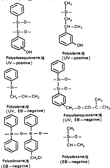
Fig. 21. Silicon containing resists
