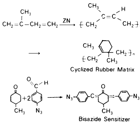
Fig. 2. Bisarylazide-rubber resists.
