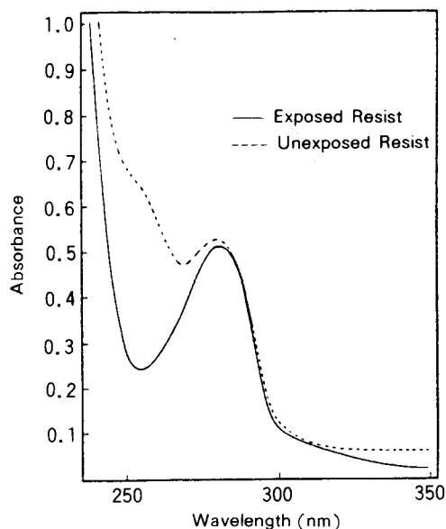
Fig. 11. Absorbance spectra of Meldrum's diazo resist before and after exposure.
