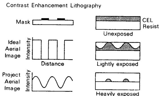
Fig. 16. A contrast enhancement lithography
