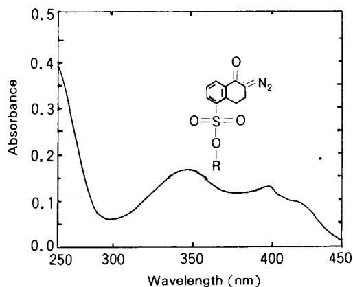
Fig. 6. Absorbance spectrum of a 1-oxo-2-diazidonaphthoquinone-5-arylsulfonate.
