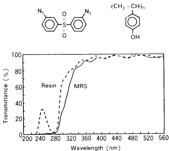
Fig. 13. Spectral transmittance of a m film of azide-phenolic resin photoresist.
