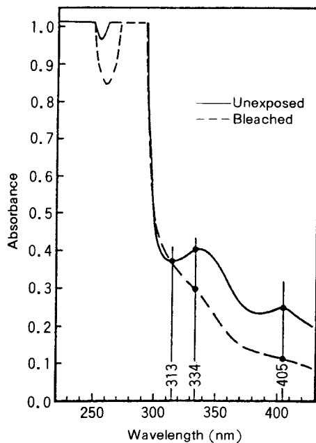
Fig. 7. Absorbance spectrum of a 1.17 \mu m film of AZ 1350J photoresist coated on quartz.
