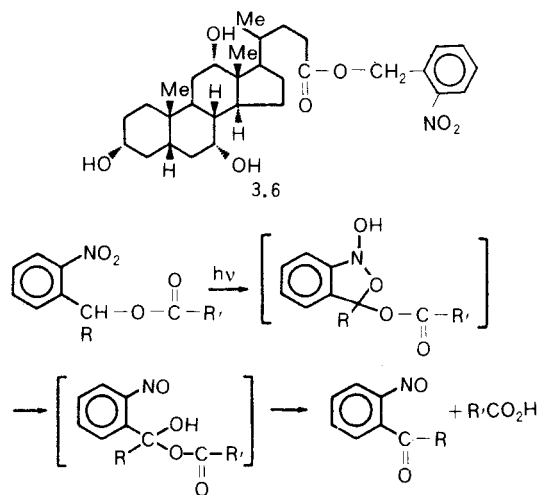
Fig. 12. Photochemical decomposition of o-nitrobenzyl ester.
