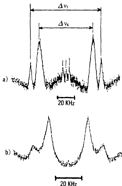
Fig. 11. DMR spectra of samples deuterium labelled on the spacer : (a) DDA9( n=10 ) ; (b) AZA9( n=7 ) : ( \Delta v_1 ) quadrupolar splitting corresponding to the deuterons in a to the ester linkage, ( \Delta v_4 ) remaining deuterons.
