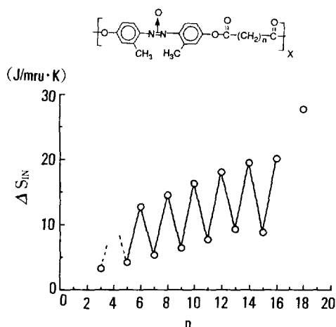
Fig. 10. The entropy of isotropization of polyesters as a function of spacer length n .
