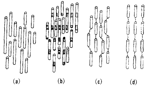
Fig. 6. (a) and (b) Nematic and smectic phases of rigidrod PLCs; (c) and (d) Nematic and smectic phases of semiflexible PLCs.
