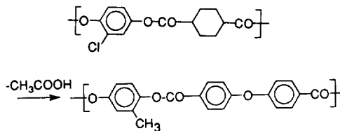
Fig. 3. Less symmetric rod-like polymers.
