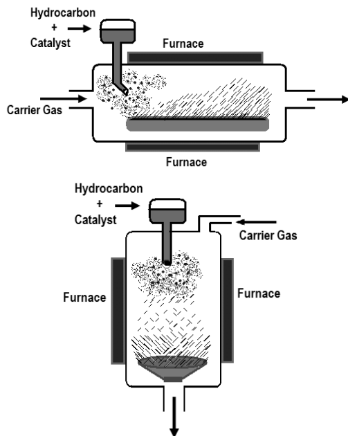
그림 12. Schematics reactors for the production of vapor grown carbon nanofibers in floating reactant methods. 31
