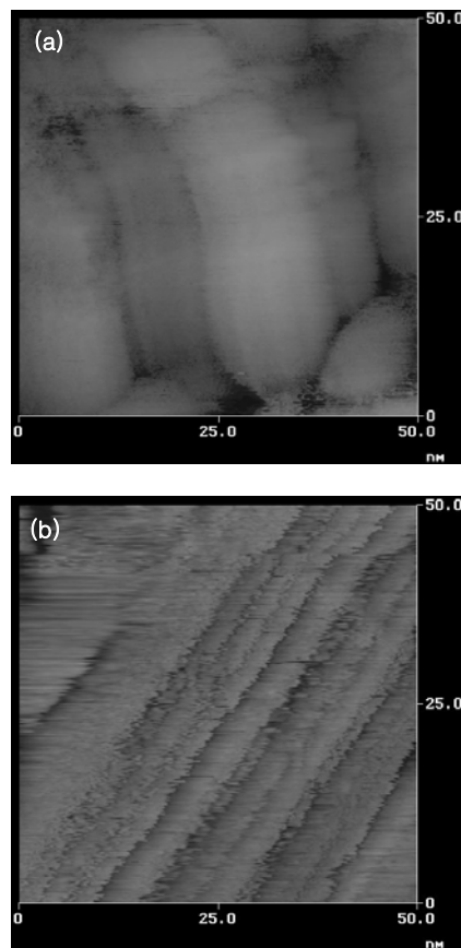
그림 3. (a) AFM image of the PAN based e-CNFs garfitized at 2,500 °C. (b) AFM image of the polyimide based e-CNFs garfitized at 2,500 °C.
