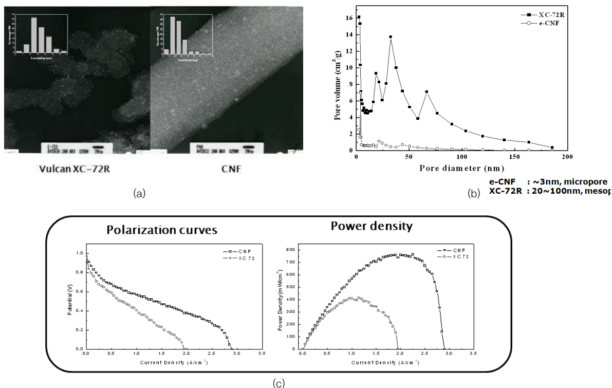
그림 9. Comparisons of the electrodes of fuel cell made from XC-72R and e-CNFs; SEM (a), pore size distributions (b), and polarization and power density curves (c). 17
