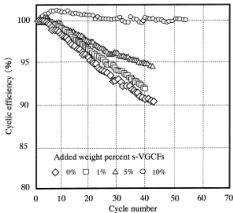
그림 15. Cyclic efficiency of synthetic graphite(HTT=2,900 °C) as a function of added weight percent of graphitized s-VGCFs, in the range 0 to 1.5 V, with a current density of 0.2 mA/cm 2 . 32,41
